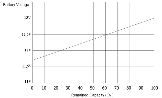
Relationship of OCV and state of charge
